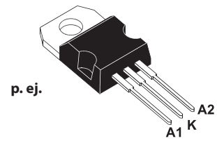
TO-220AB STPS30L40CT
